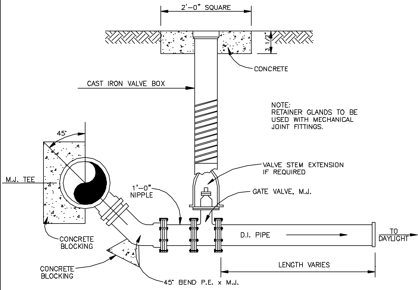
BLOW-OFF ASSEMBLY NOT TO SCALE
