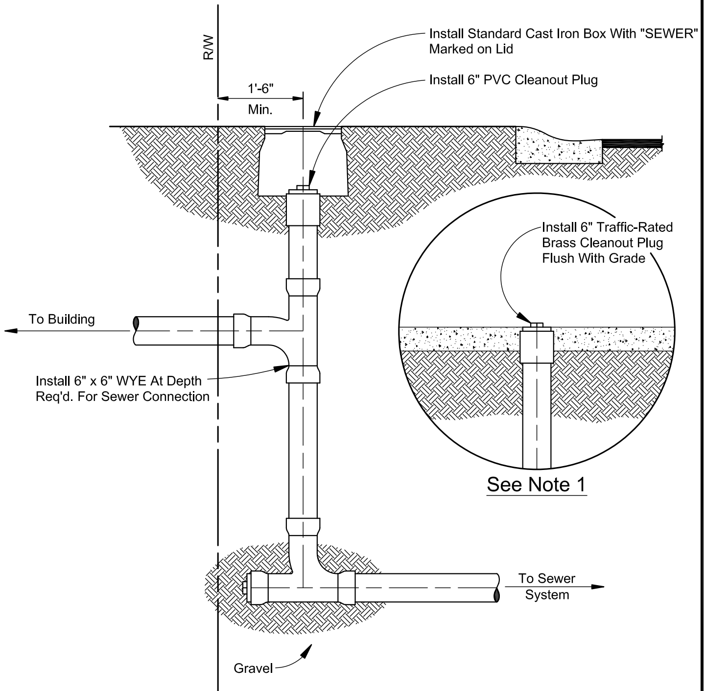
Cleanout Detail (By Builder)
